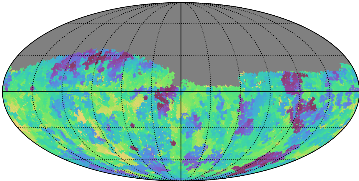
baseline_v3.0_10yrs Yr 1 g band: Min fiveSigmaDepth
