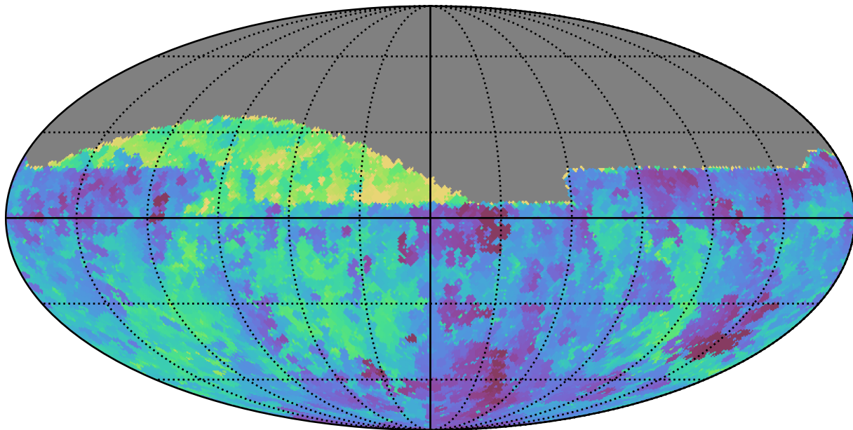
baseline_v3.0_10yrs Yr 1 all bands: Min fiveSigmaDepth
