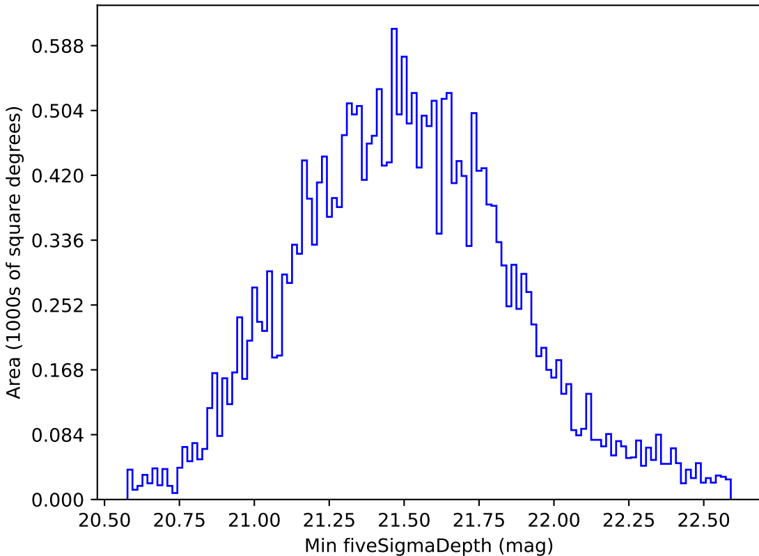
baseline_v3.0_10yrs Yr 1 all bands: Min fiveSigmaDepth
