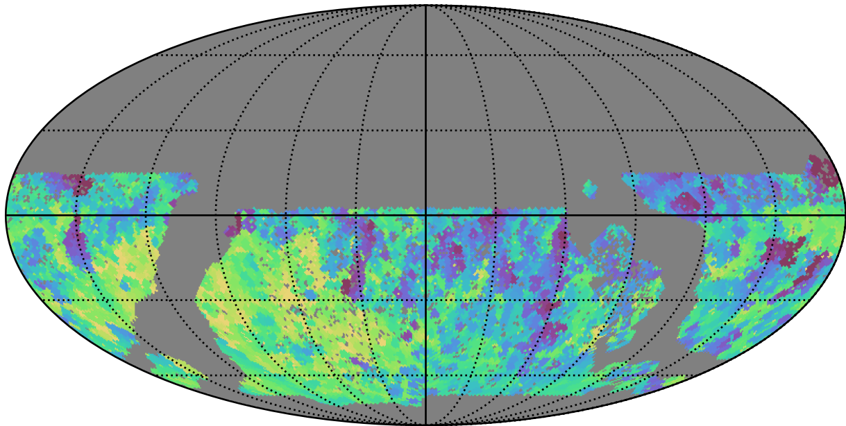
baseline_v3.0_10yrs WFD z band: Min fiveSigmaDepth
