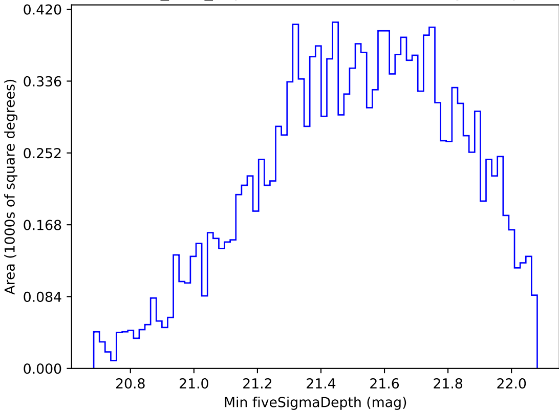
baseline_v3.0_10yrs WFD z band: Min fiveSigmaDepth
