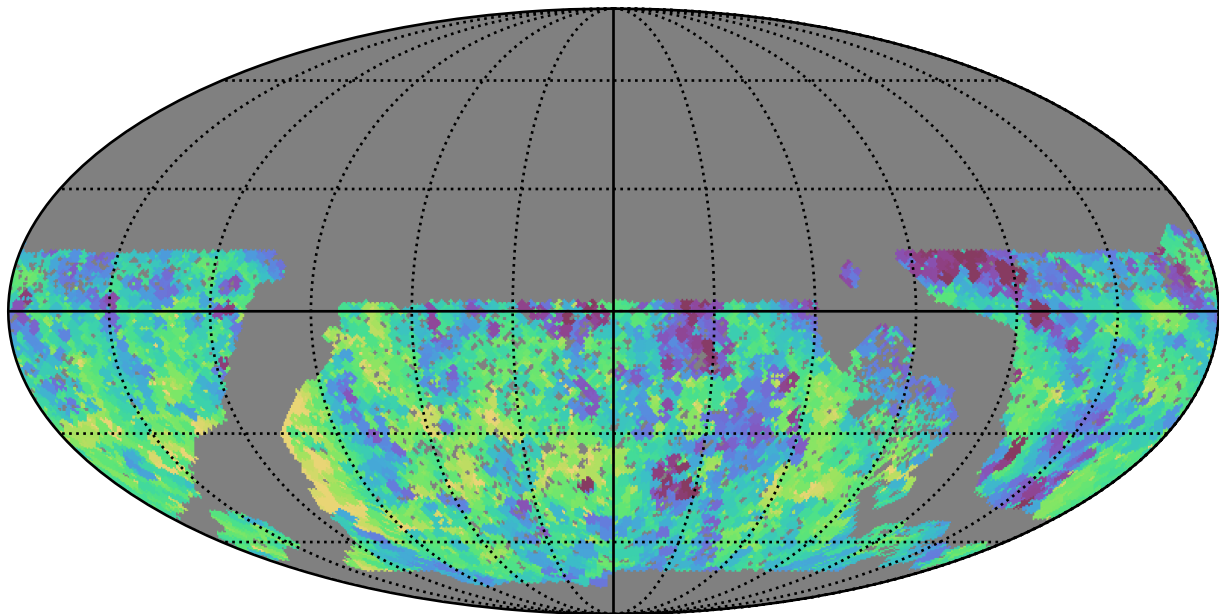
baseline_v3.0_10yrs WFD y band: Min fiveSigmaDepth
