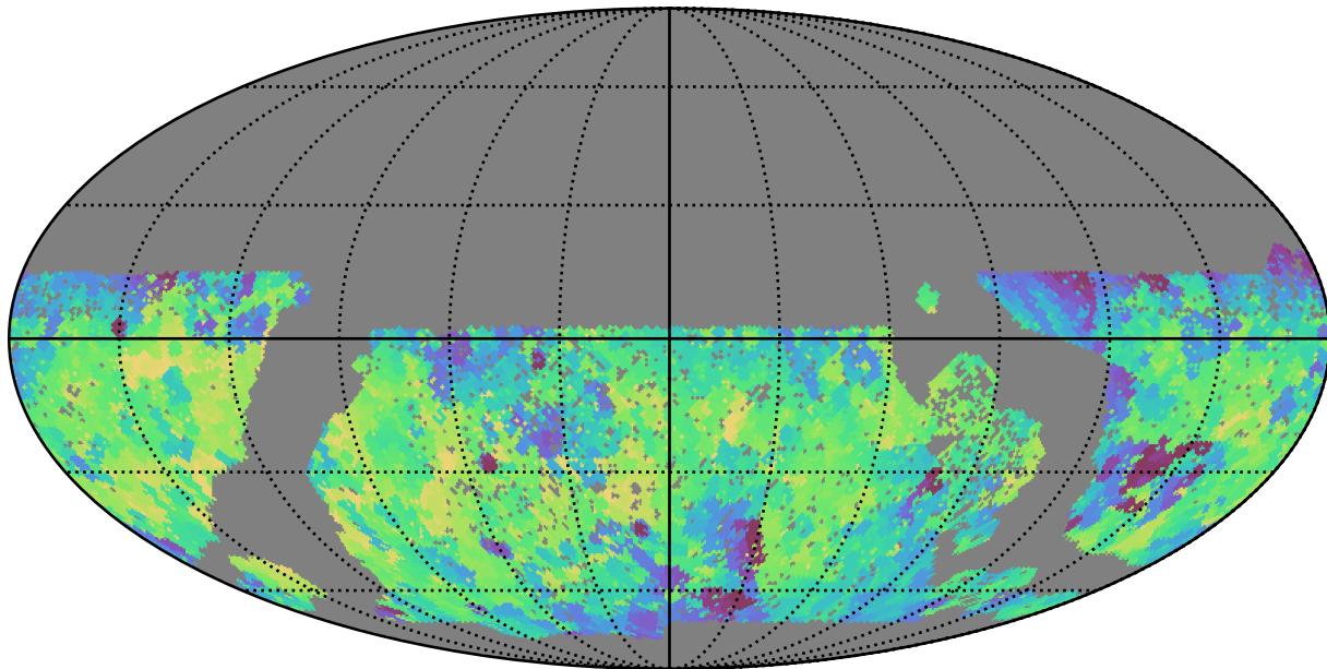
baseline_v3.0_10yrs WFD u band: Min fiveSigmaDepth
