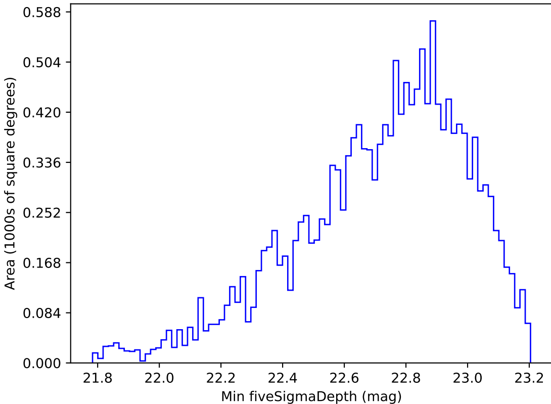
baseline_v3.0_10yrs WFD u band: Min fiveSigmaDepth
