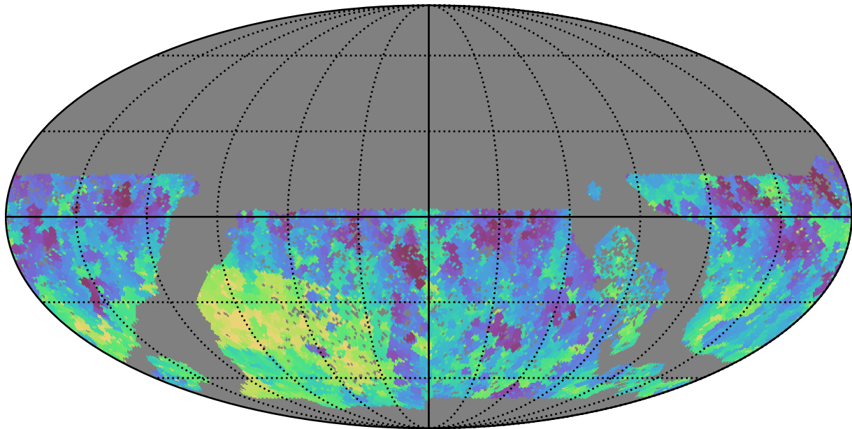
baseline_v3.0_10yrs WFD r band: Min fiveSigmaDepth
