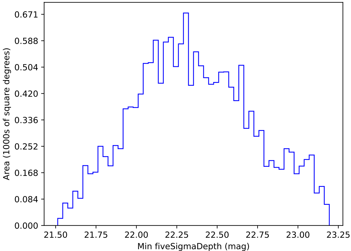
baseline_v3.0_10yrs WFD r band: Min fiveSigmaDepth
