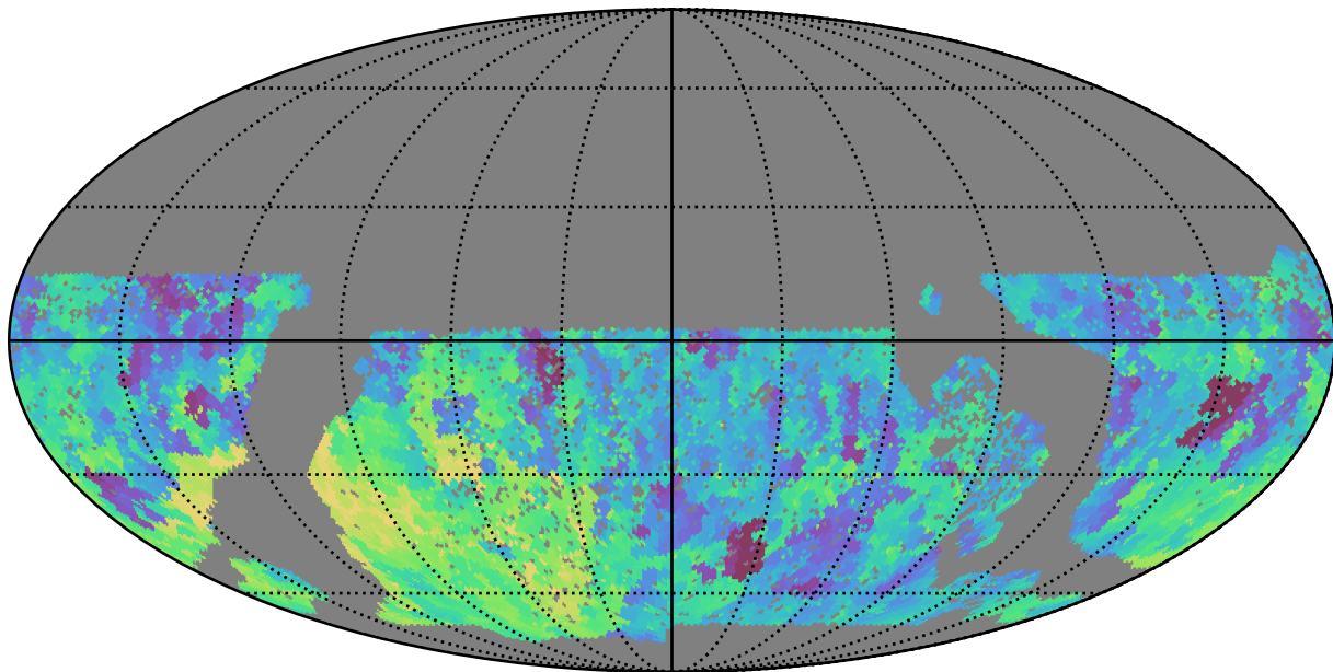
baseline_v3.0_10yrs WFD i band: Min fiveSigmaDepth
