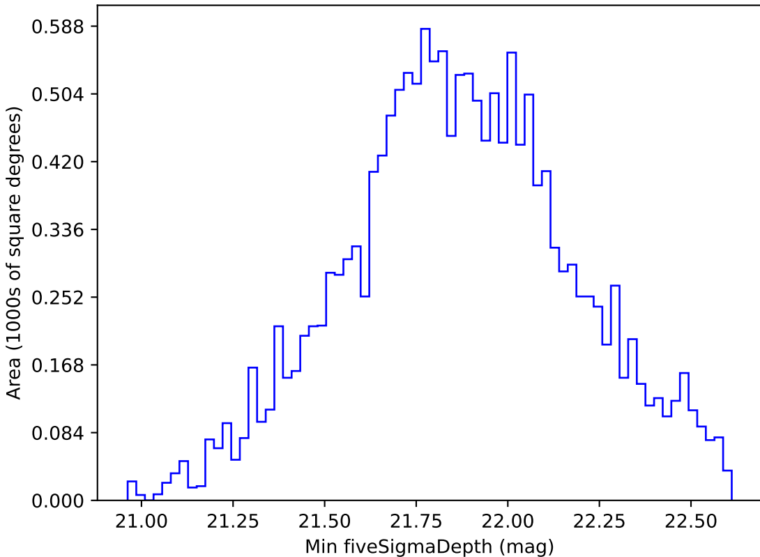
baseline_v3.0_10yrs WFD i band: Min fiveSigmaDepth
