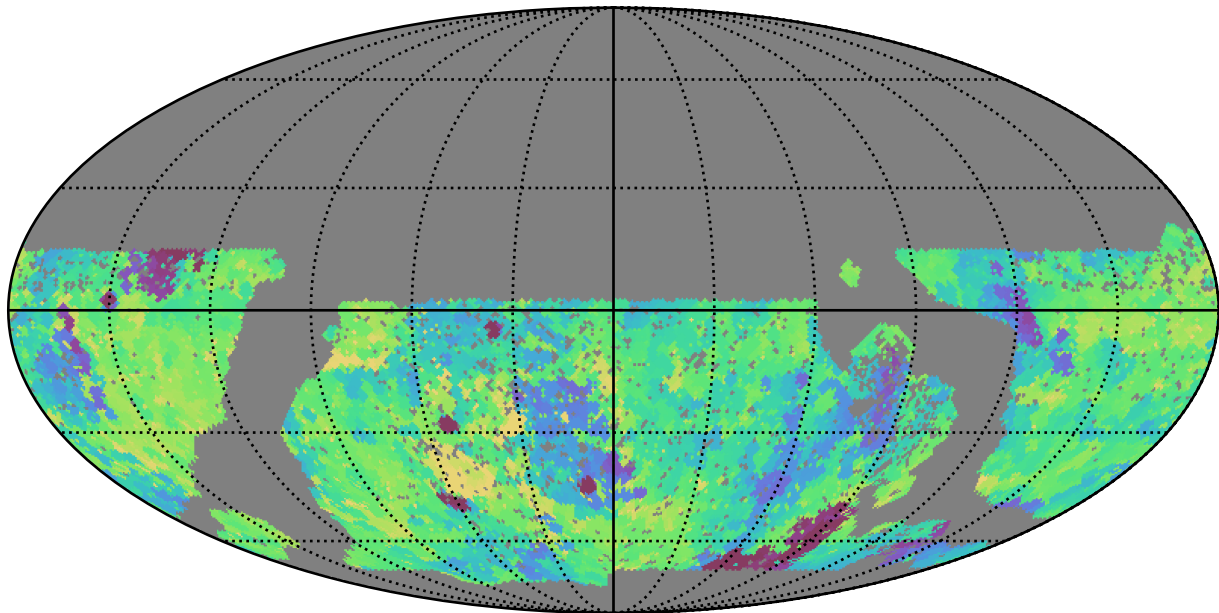
baseline_v3.0_10yrs WFD g band: Min fiveSigmaDepth
