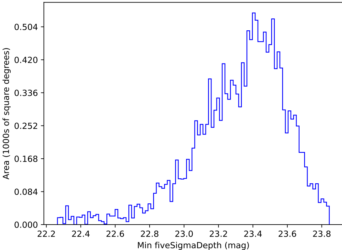
baseline_v3.0_10yrs WFD g band: Min fiveSigmaDepth
