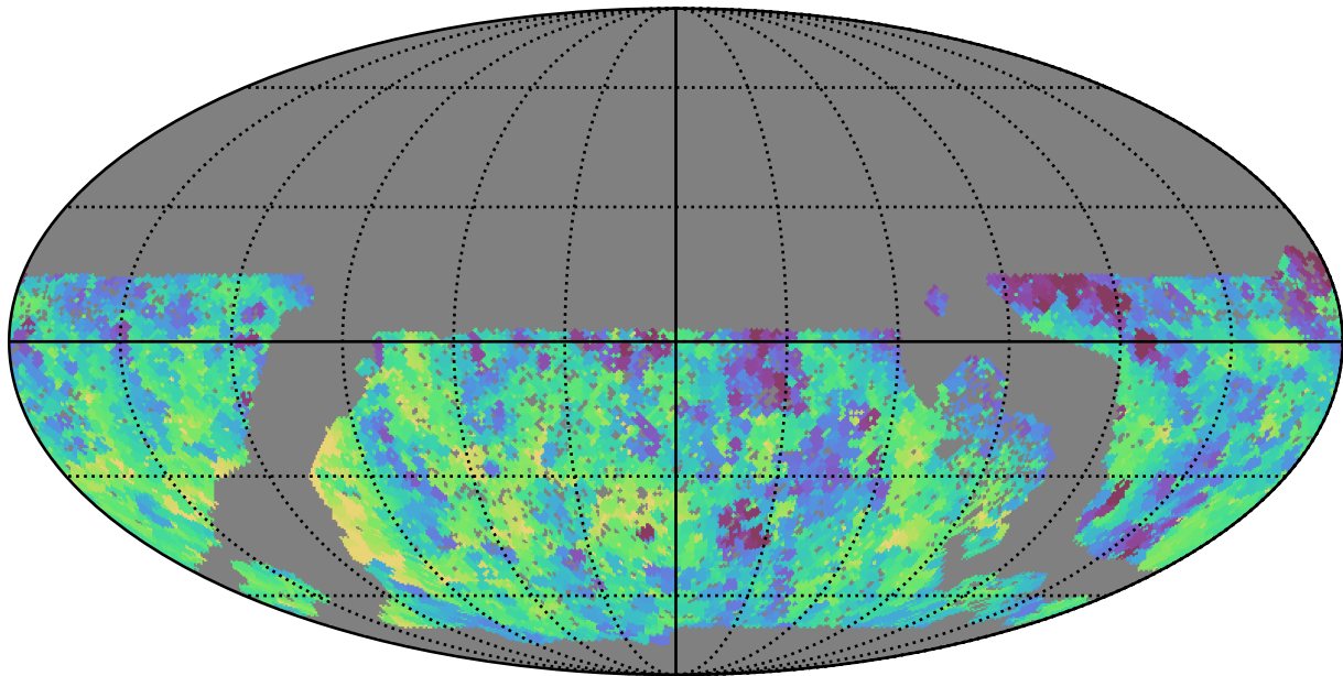
baseline_v3.0_10yrs WFD all bands: Min fiveSigmaDepth
