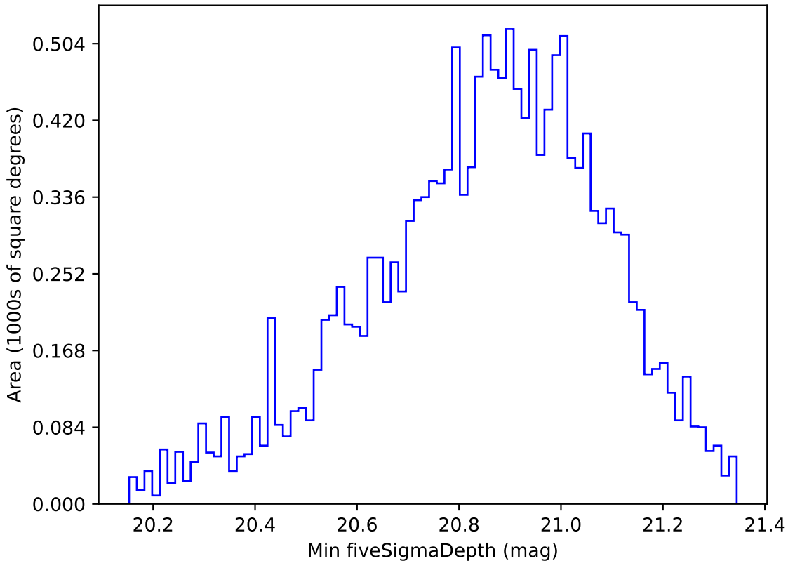
baseline_v3.0_10yrs WFD all bands: Min fiveSigmaDepth
