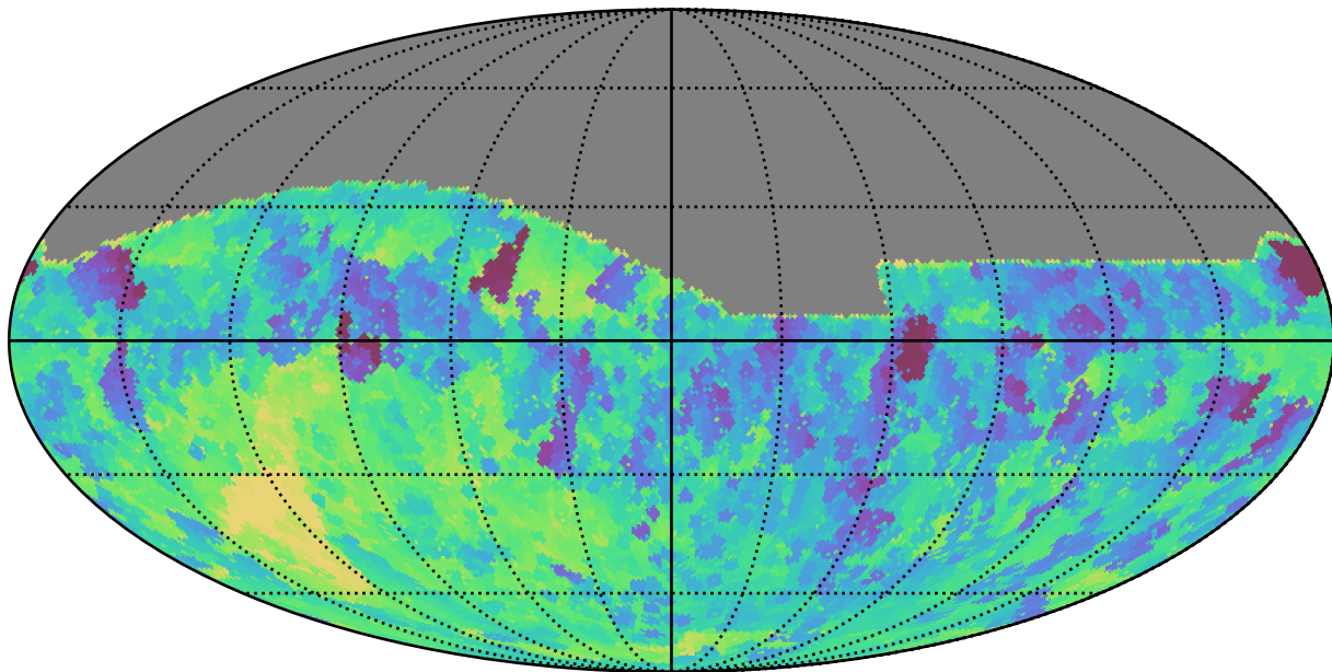
baseline_v3.0_10yrs All sky z band: Min fiveSigmaDepth
