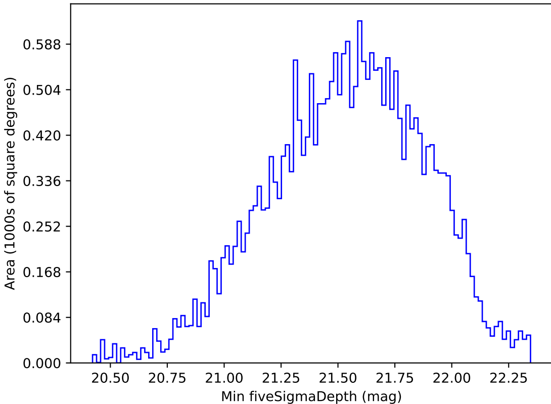
baseline_v3.0_10yrs All sky z band: Min fiveSigmaDepth
