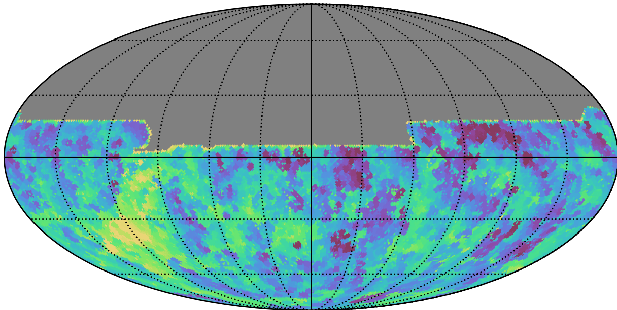
baseline_v3.0_10yrs All sky y band: Min fiveSigmaDepth
