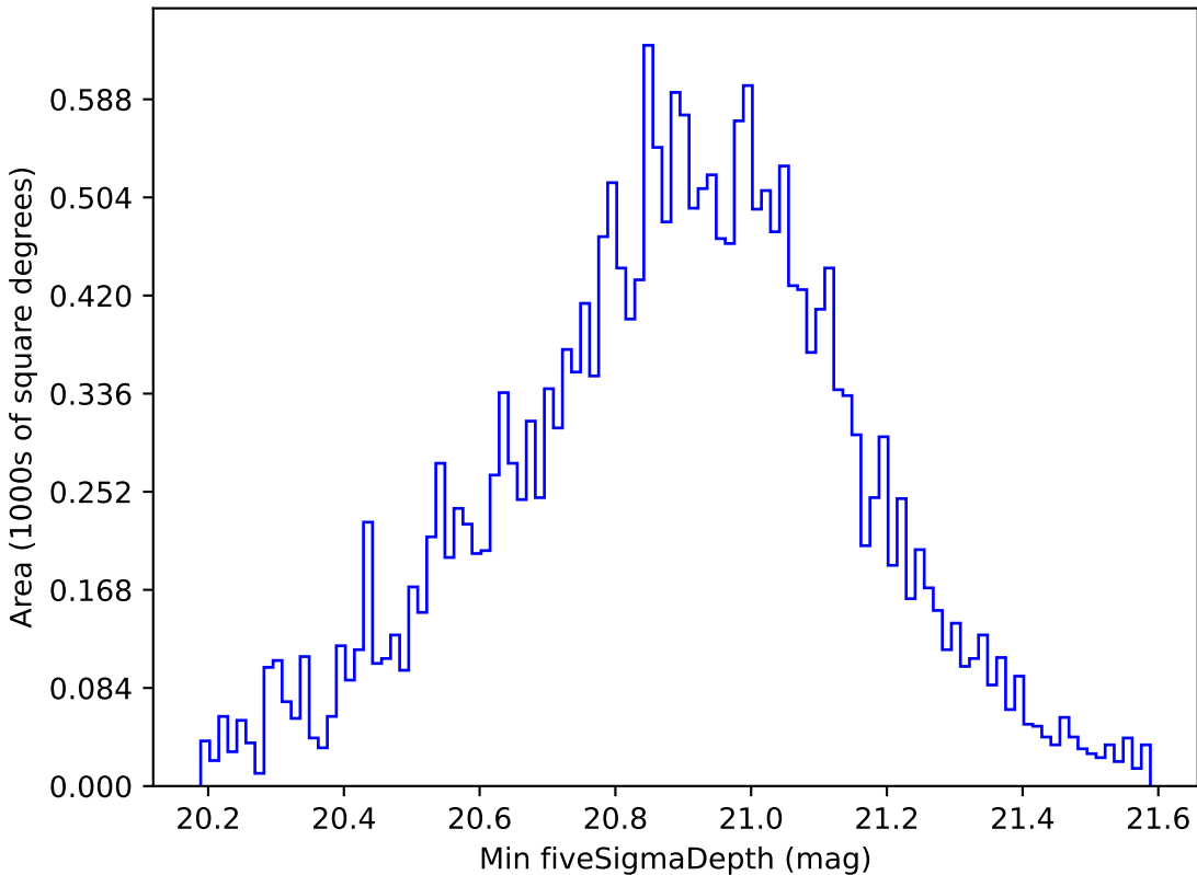
baseline_v3.0_10yrs All sky y band: Min fiveSigmaDepth
