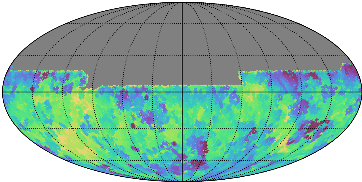
baseline_v3.0_10yrs All sky u band: Min fiveSigmaDepth
