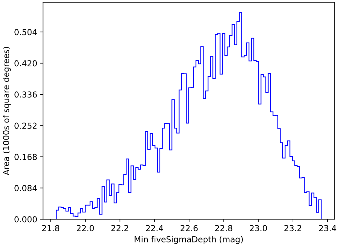
baseline_v3.0_10yrs All sky u band: Min fiveSigmaDepth
