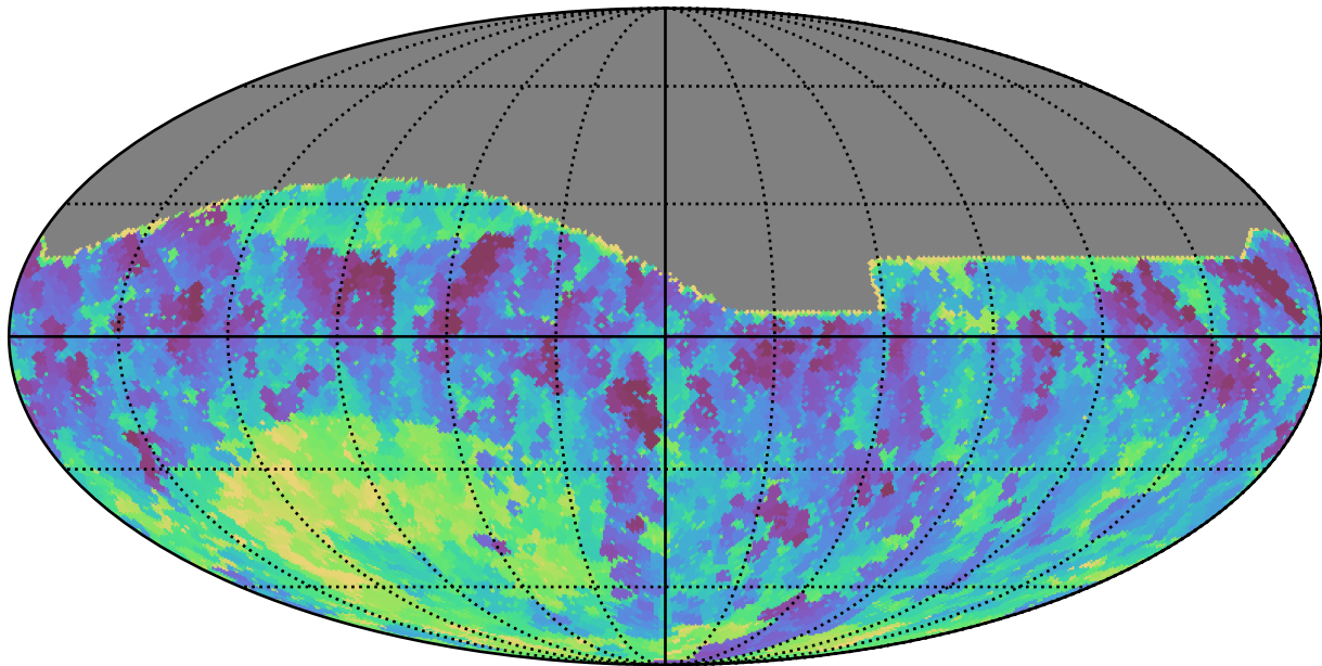
baseline_v3.0_10yrs All sky r band: Min fiveSigmaDepth
