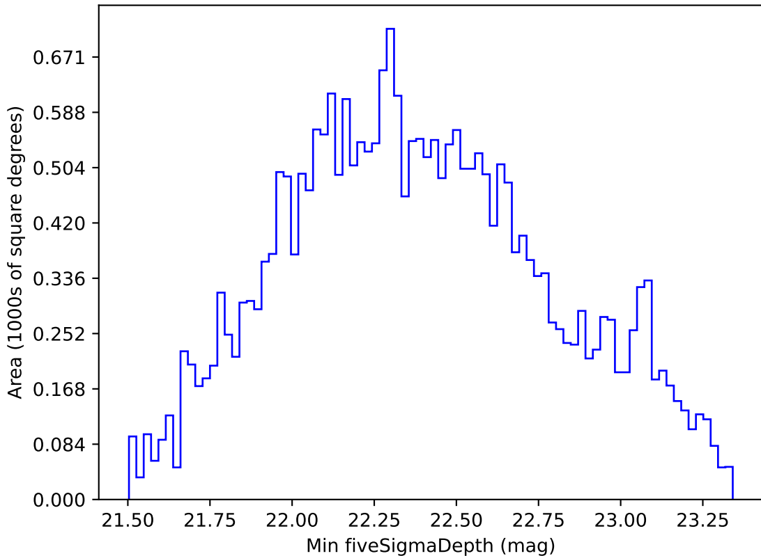
baseline_v3.0_10yrs All sky r band: Min fiveSigmaDepth
