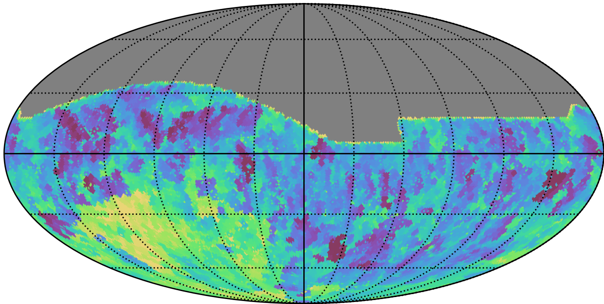
baseline_v3.0_10yrs All sky i band: Min fiveSigmaDepth
