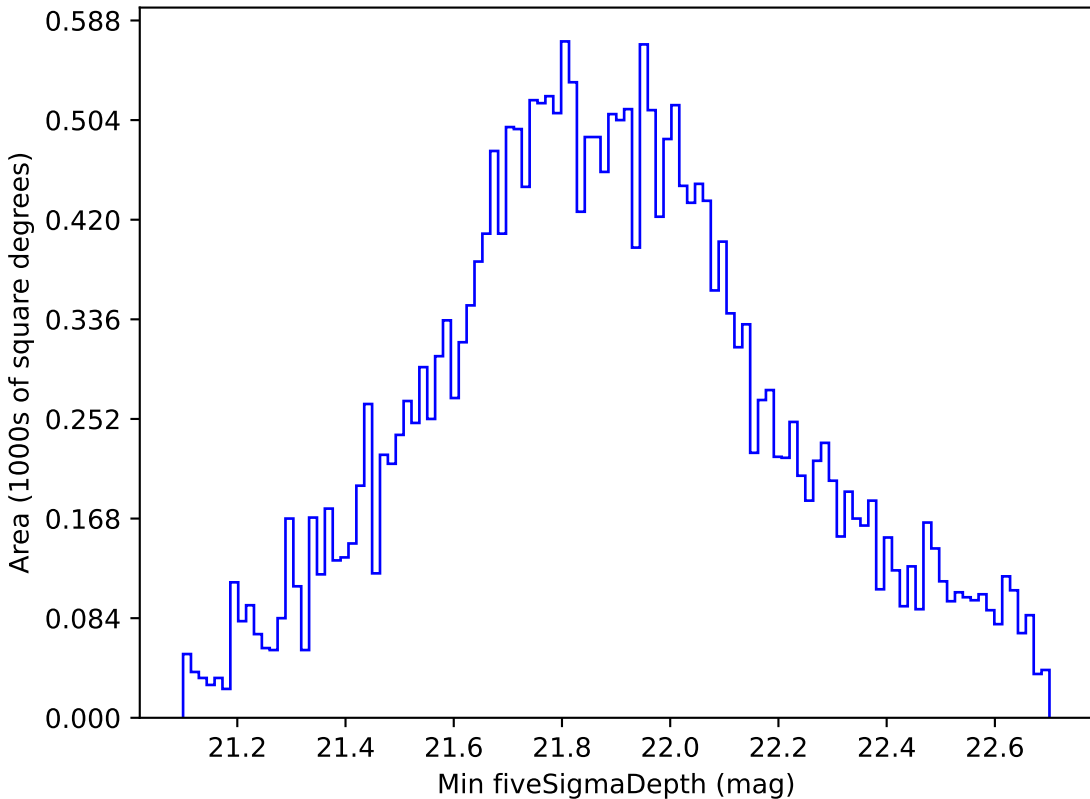
baseline_v3.0_10yrs All sky i band: Min fiveSigmaDepth
