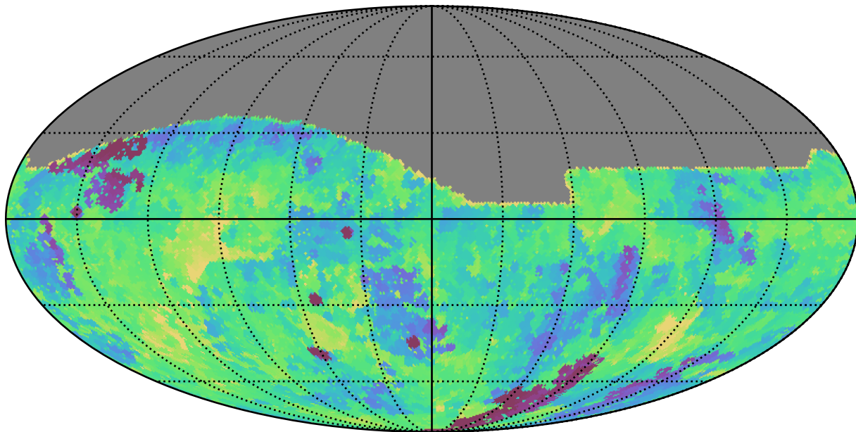
baseline_v3.0_10yrs All sky g band: Min fiveSigmaDepth
