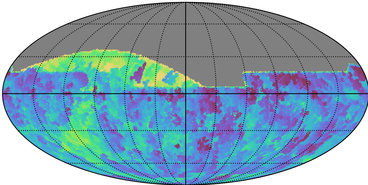
baseline_v3.0_10yrs All sky all bands: Min fiveSigmaDepth
