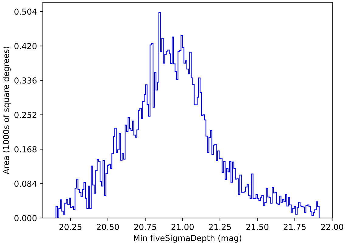
baseline_v3.0_10yrs All sky all bands: Min fiveSigmaDepth
