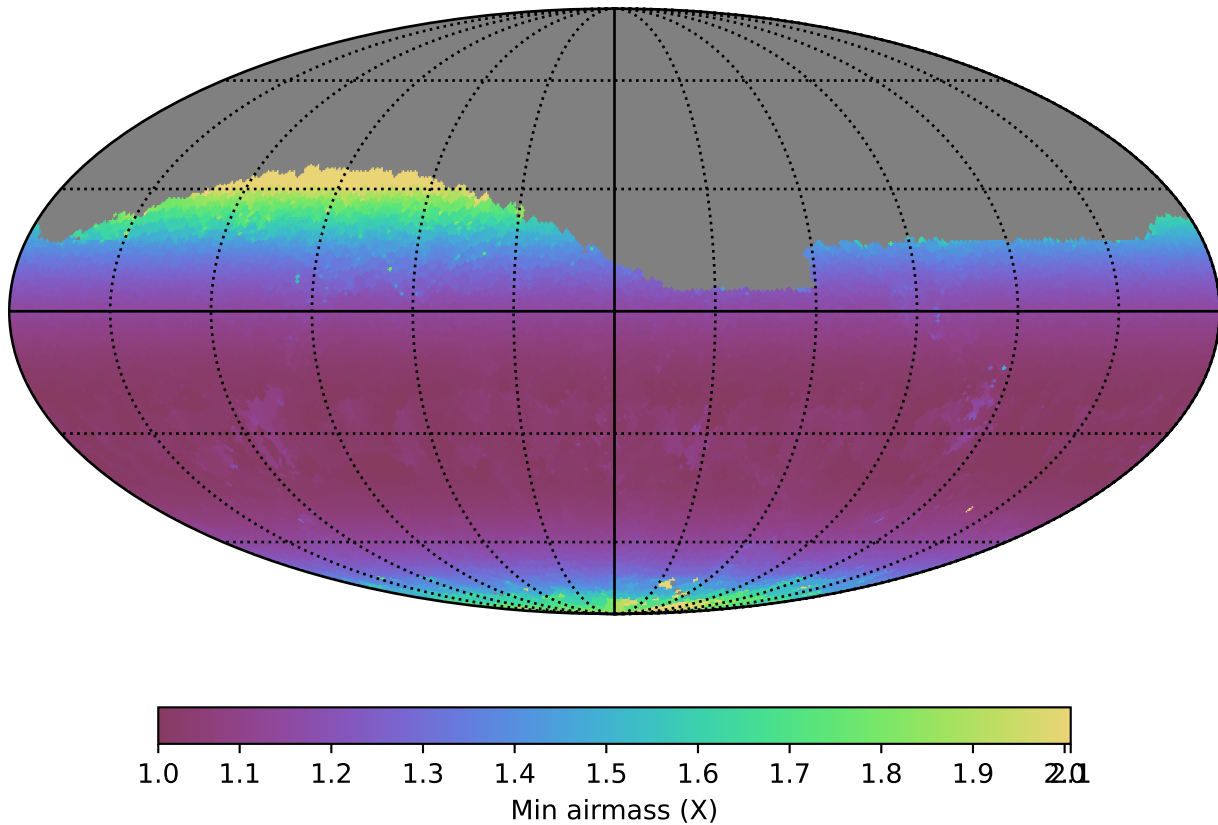
baseline_v3.0_10yrs Yr 1 z band: Min airmass
