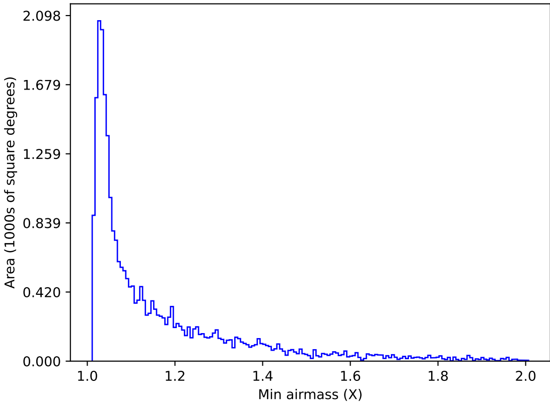
baseline_v3.0_10yrs Yr 1 z band: Min airmass
