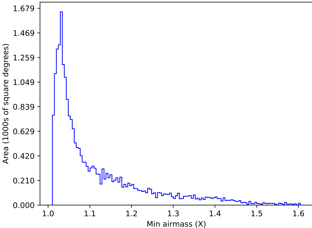
baseline_v3.0_10yrs Yr 1 y band: Min airmass
