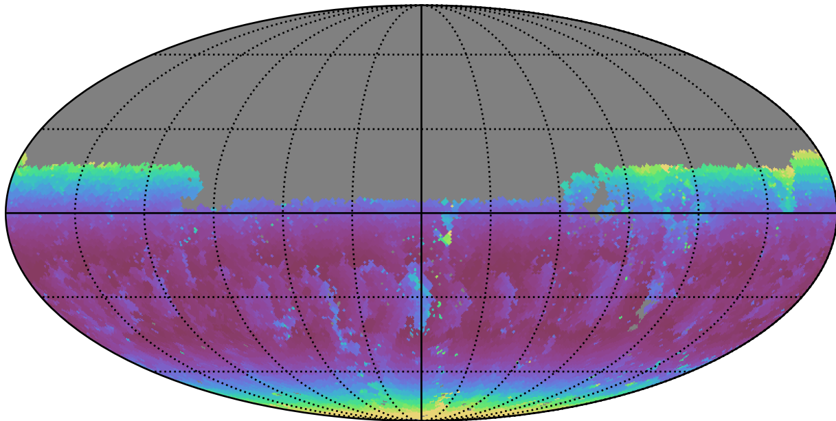
baseline_v3.0_10yrs Yr 1 u band: Min airmass
