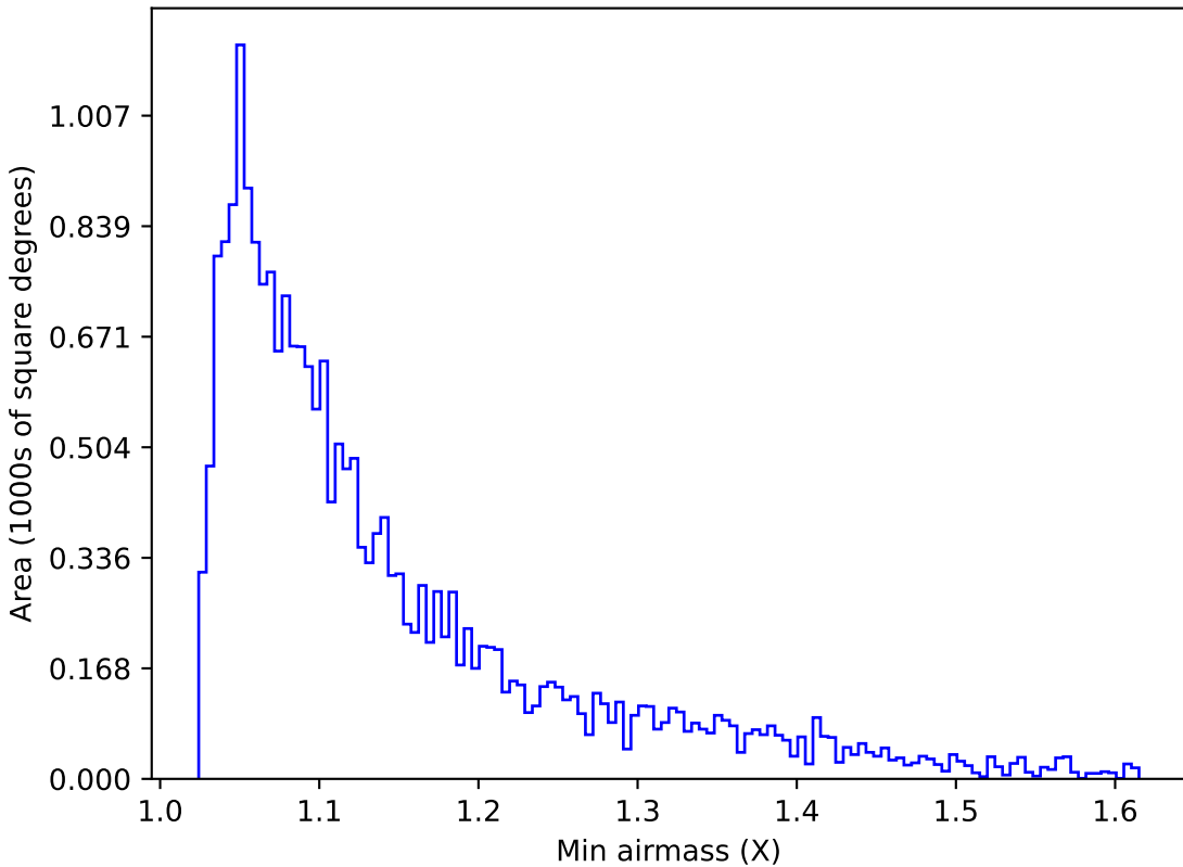
baseline_v3.0_10yrs Yr 1 u band: Min airmass
