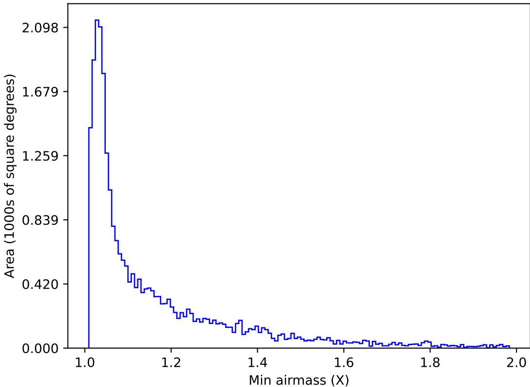
baseline_v3.0_10yrs Yr 1 r band: Min airmass
