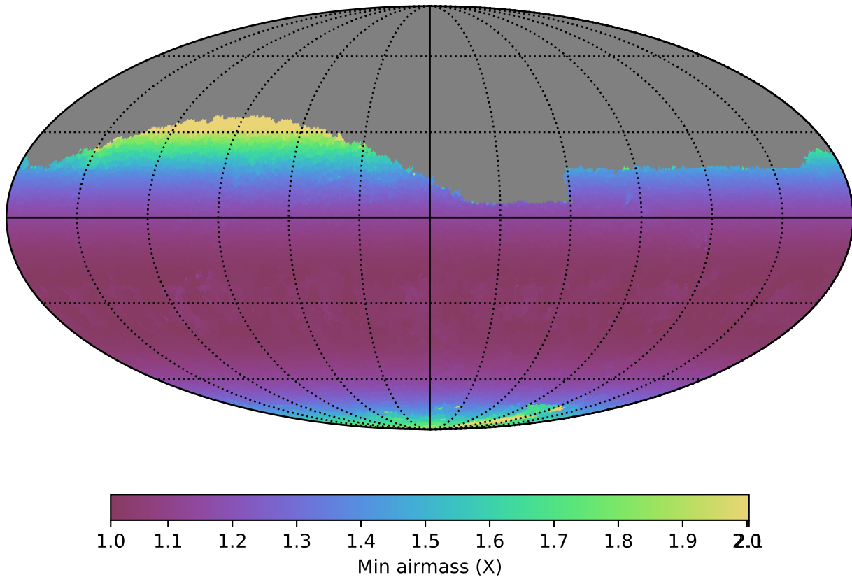
baseline_v3.0_10yrs Yr 1 i band: Min airmass
