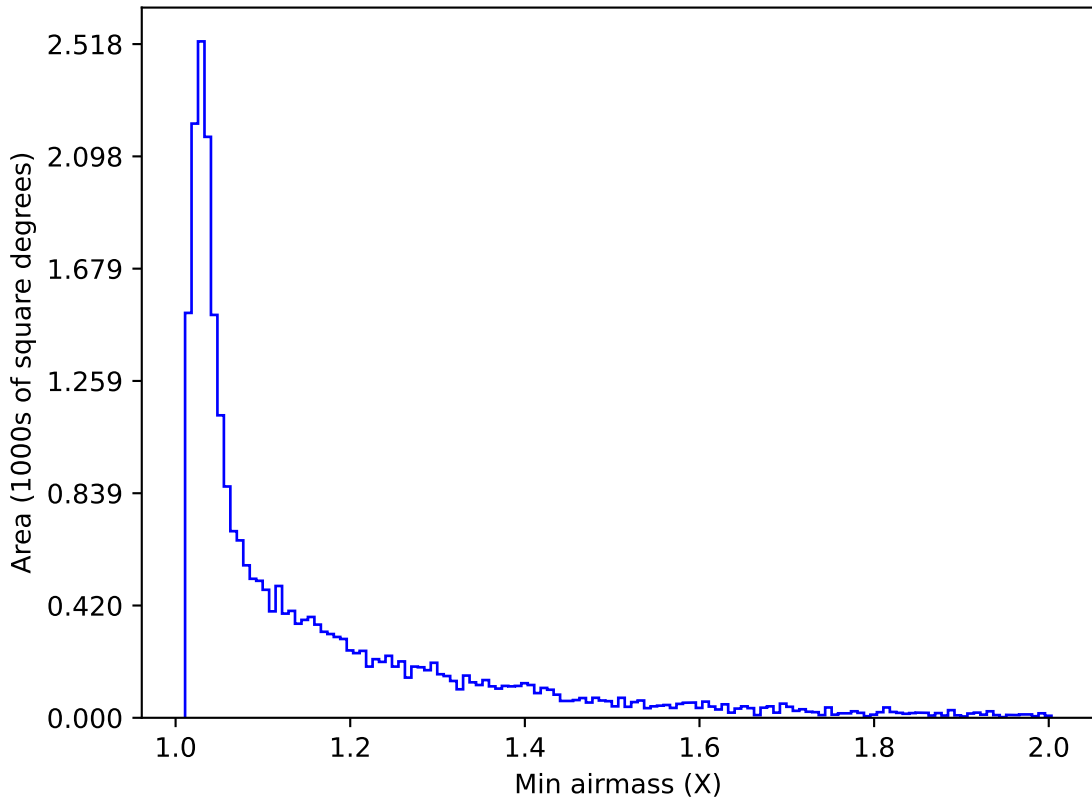
baseline_v3.0_10yrs Yr 1 i band: Min airmass
