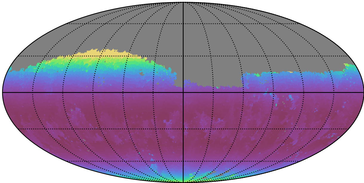
baseline_v3.0_10yrs Yr 1 g band: Min airmass
