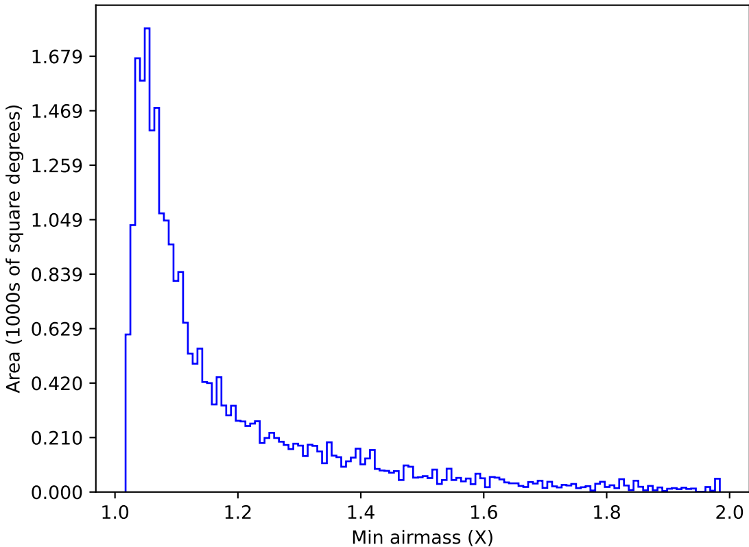
baseline_v3.0_10yrs Yr 1 g band: Min airmass
