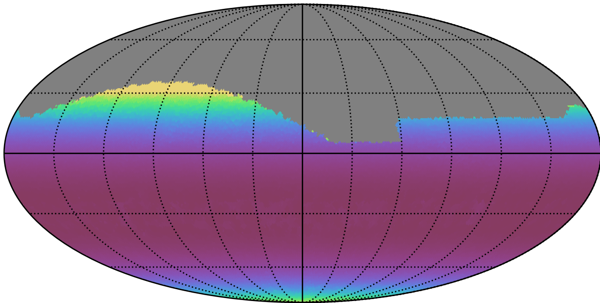
baseline_v3.0_10yrs Yr 1 all bands: Min airmass
