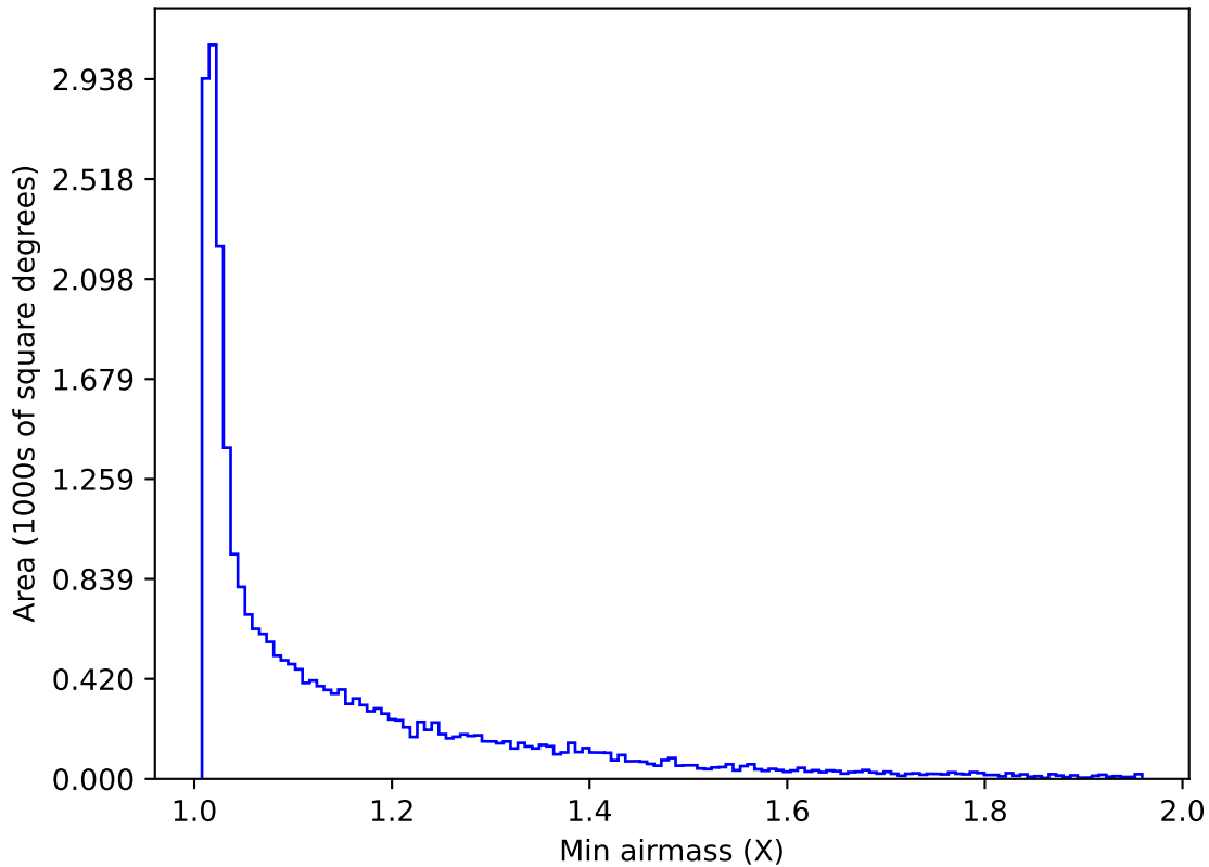
baseline_v3.0_10yrs Yr 1 all bands: Min airmass
