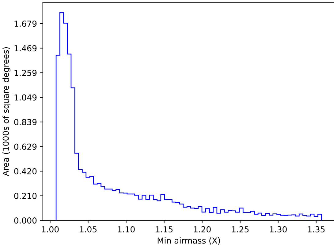
baseline_v3.0_10yrs WFD z band: Min airmass
