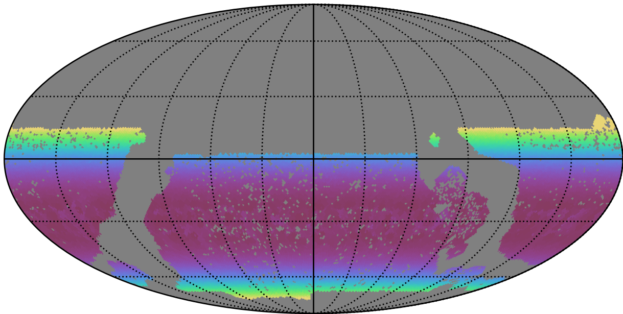
baseline_v3.0_10yrs WFD y band: Min airmass
