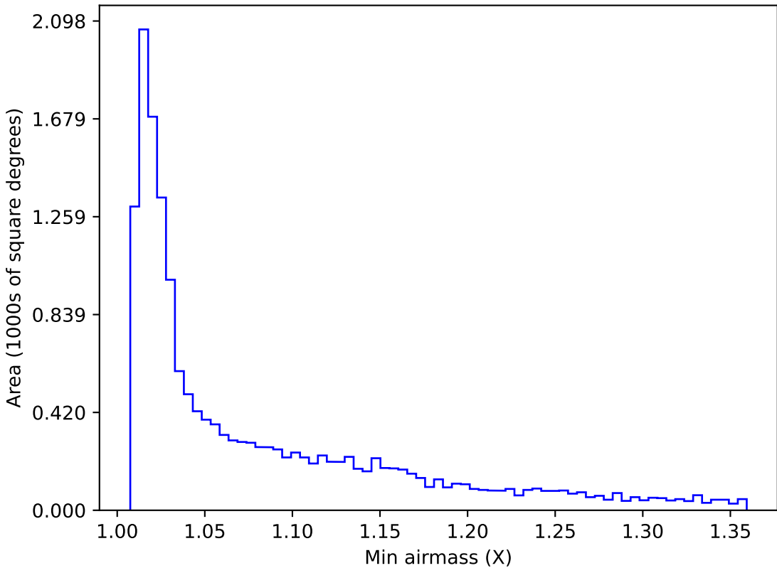
baseline_v3.0_10yrs WFD y band: Min airmass
