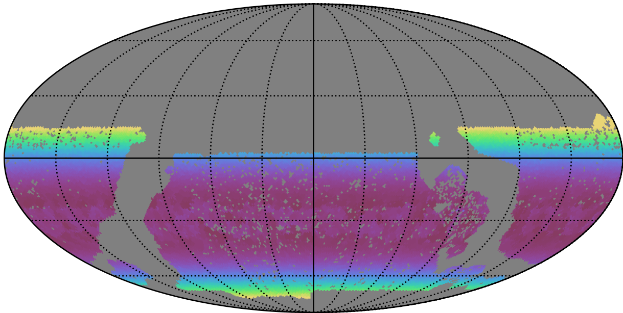
baseline_v3.0_10yrs WFD u band: Min airmass
