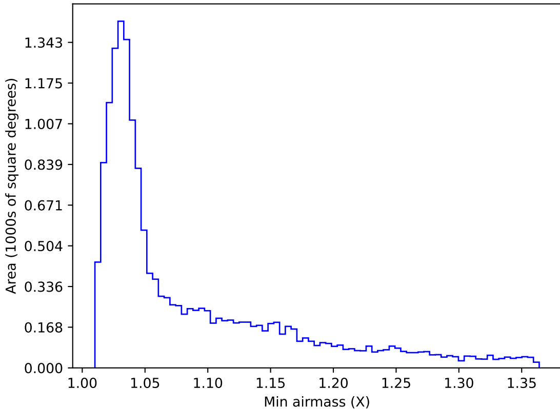
baseline_v3.0_10yrs WFD u band: Min airmass
