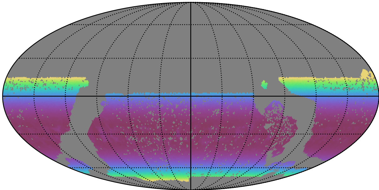
baseline_v3.0_10yrs WFD r band: Min airmass
