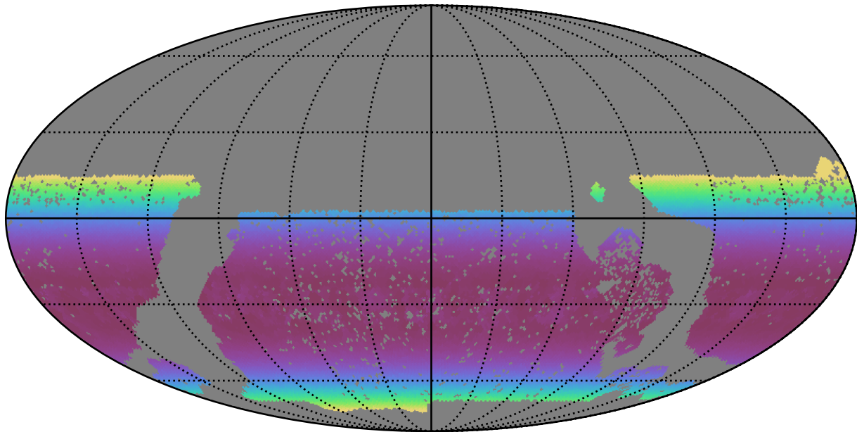
baseline_v3.0_10yrs WFD i band: Min airmass
