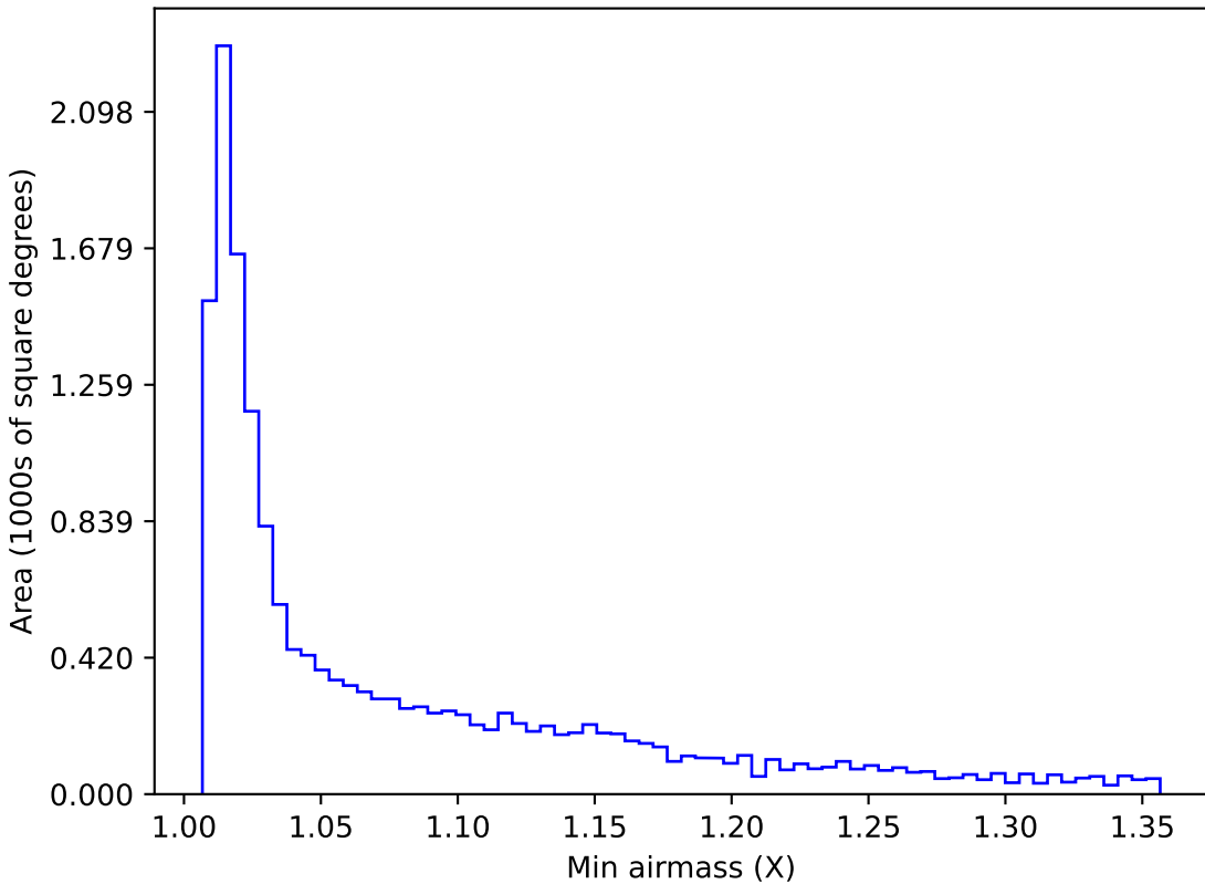
baseline_v3.0_10yrs WFD i band: Min airmass
