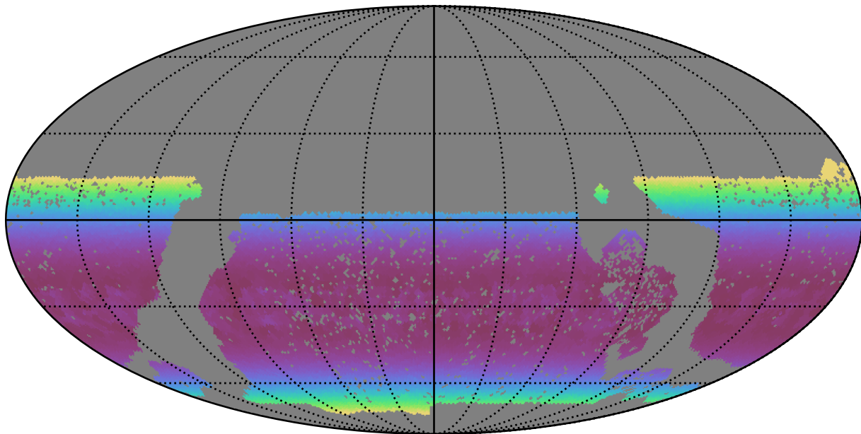
baseline_v3.0_10yrs WFD g band: Min airmass
